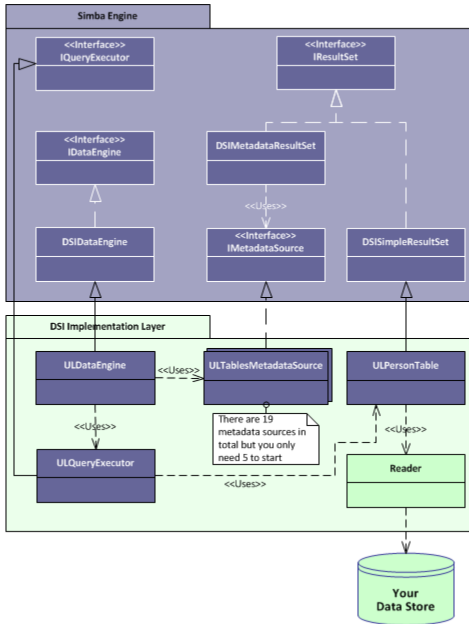
Figure 1: Design pattern for a DSI implementation.
